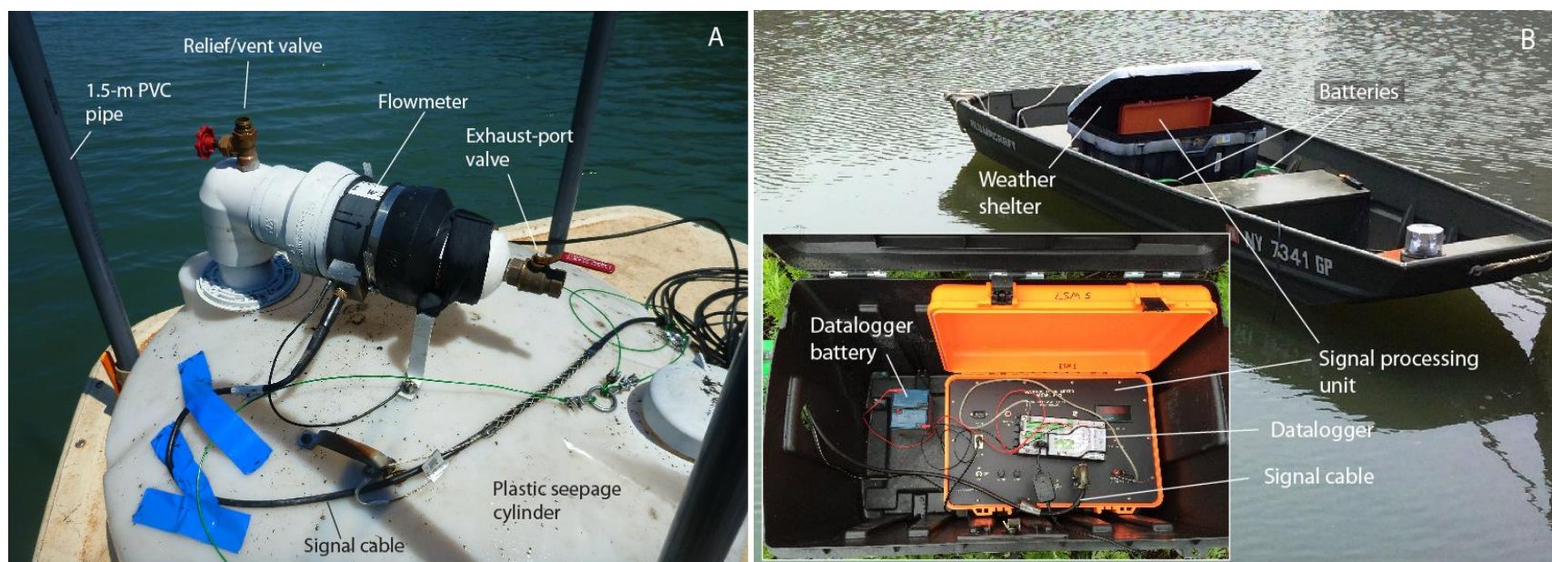
Figure 3. Photos of an electromagnetic seepage meter deployed at Newton Creek. A, Seepage cylinder and flowmeter prior to being lowered onto the sediment bed; photograph also shows the three polyvinyl chloride (PVC) pipes that will be pushed into the sediment by a diver. B, Signal-processing unit in an anchored boat; inset photograph shows close-up of weather shelter interior.
