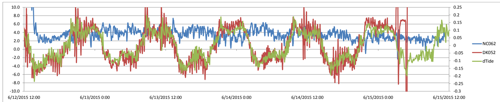
Figure 23. Smoothed seepage measured at DK052 and NC062, in centimeters per day (cm/d), with the previous tidal value minus the current tidal value (dTide), in feet, plotted on the right axis.
