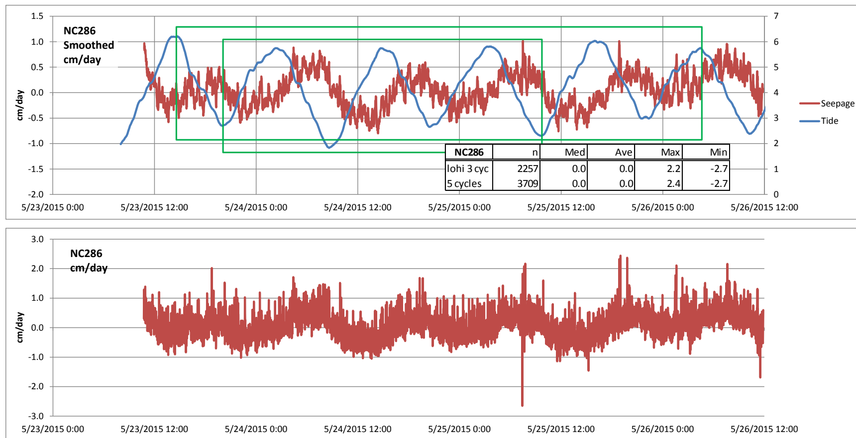
Figure 14. Seepage measured each minute during deployment at NC286, in centimeters per day. The upper plot displays smoothed data based on a 7-minute moving average, with relative tide, in feet, plotted on the right axis. The lower plot presents the actual 1-minute values. The green rectangles indicate the duration of the data-summary periods. In the inset table, “lo hi” indicates one complete tidal cycle beginning and ending with low tide, and “3 cyc” and “5 cycles” indicate the number of tidal cycles during which seepage was measured. (cm/d, centimeters per day; n, number of 1-minute values; Med, median of n values; Ave, average of n values; Max, maximum of n values; Min, minimum of n values; cyc, cycles)
