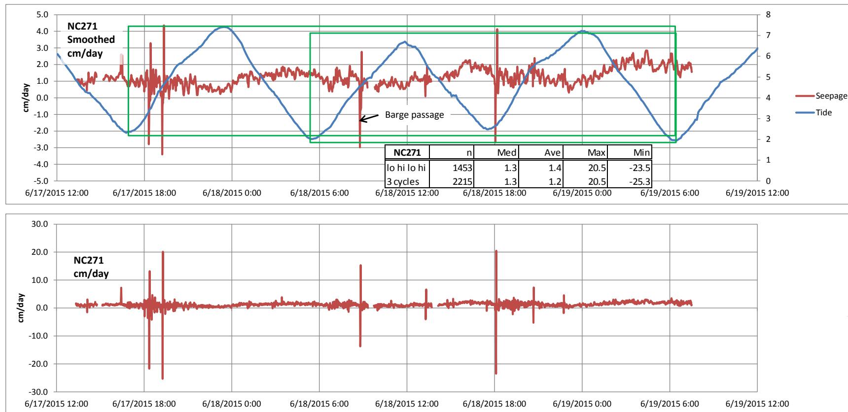
Figure 28. Seepage measured each minute during deployment at NC271, in centimeters per day. The upper plot displays smoothed data based on a 7-minute moving average, with relative tide, in feet, plotted on the right axis. The lower plot presents the actual 1-minute values. The green rectangles indicate the duration of the data-summary periods. In the inset table, “lo hi lo hi” indicates two complete tidal cycles beginning and ending with low tide, and “3 cycles” indicates that seepage was measured over three tidal cycles. (cm/d, centimeters per day; n, number of 1-minute values; Med, median of n values; Ave, average of n values; Max, maximum of n values; Min, minimum of n values)
