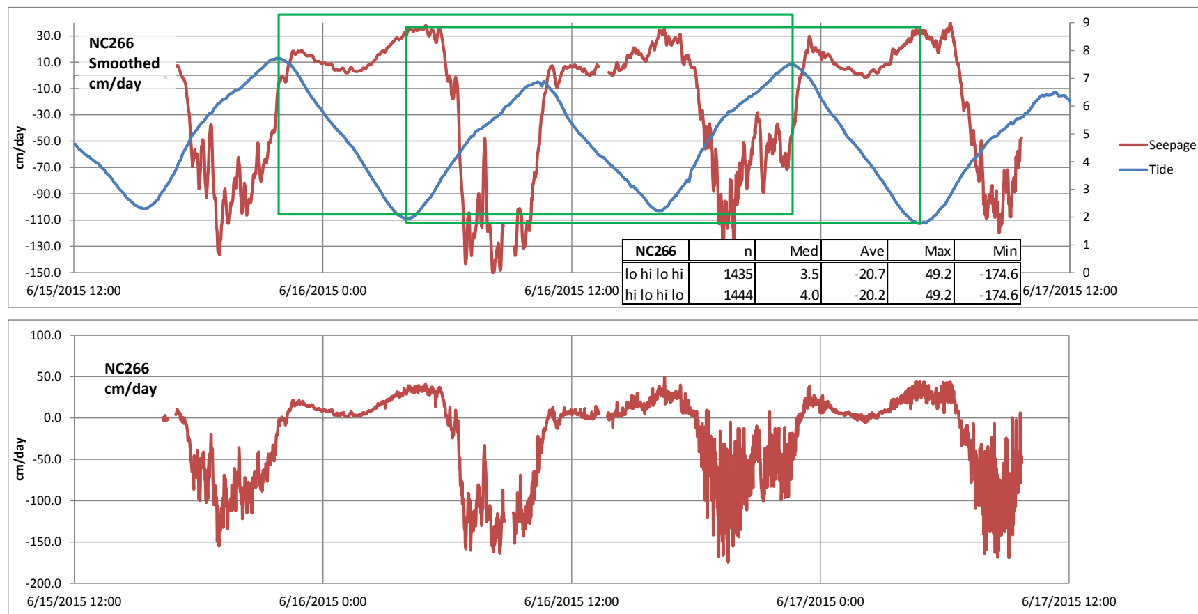
Figure 26. Seepage measured each minute during deployment at NC266, in centimeters per day. The upper plot displays smoothed data based on a 7-minute moving average, with relative tide, in feet, plotted on the right axis. The lower plot presents the actual 1-minute values. The green rectangles indicate the duration of the data-summary periods. In the inset table, “lo hi” indicates one complete tidal cycle beginning and ending with low tide, and “hi lo” indicates one complete tidal cycle beginning and ending with high tide. (cm/d, centimeters per day; n, number of 1-minute values; Med, median of n values; Ave, average of n values; Max, maximum of n values; Min, minimum of n values; cyc, cycles)
