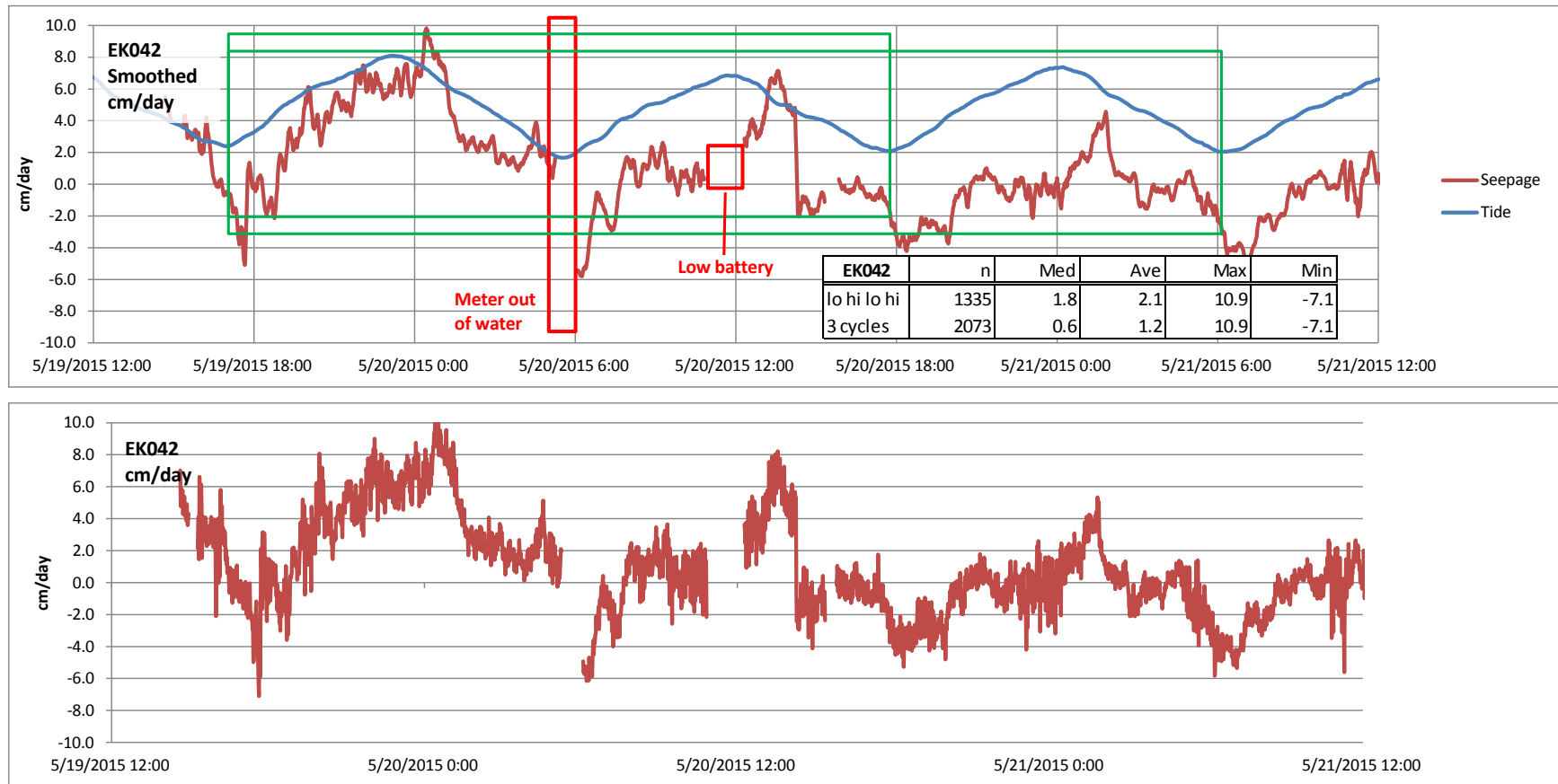
Figure 6. Seepage measured each minute during deployment at EK042, in centimeters per day. The upper plot displays smoothed data based on a 7-minute moving average and relative tide in feet. The lower plot presents the actual 1-minute values. The green rectangles indicate the duration of the data-summary periods. In the inset table, “lo hi lo hi” indicates two complete tidal cycles beginning and ending with low tide, and “3 cycles” indicates that seepage was measured over three tidal cycles. (cm/d, centimeters per day; n, number of 1-minute values; Med, median of n values; Ave, average of n values; Max, maximum of n values; Min, minimum of n values)
